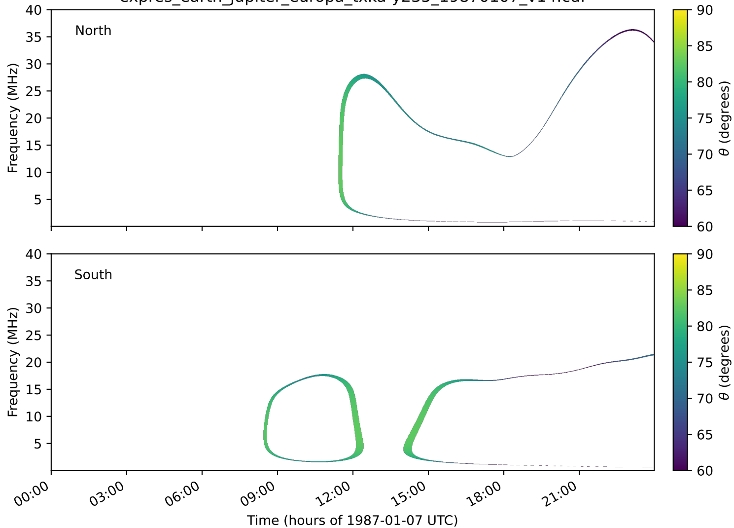
expres_earth_jupiter_europa_txka-y235_19870107_v14.cdf
