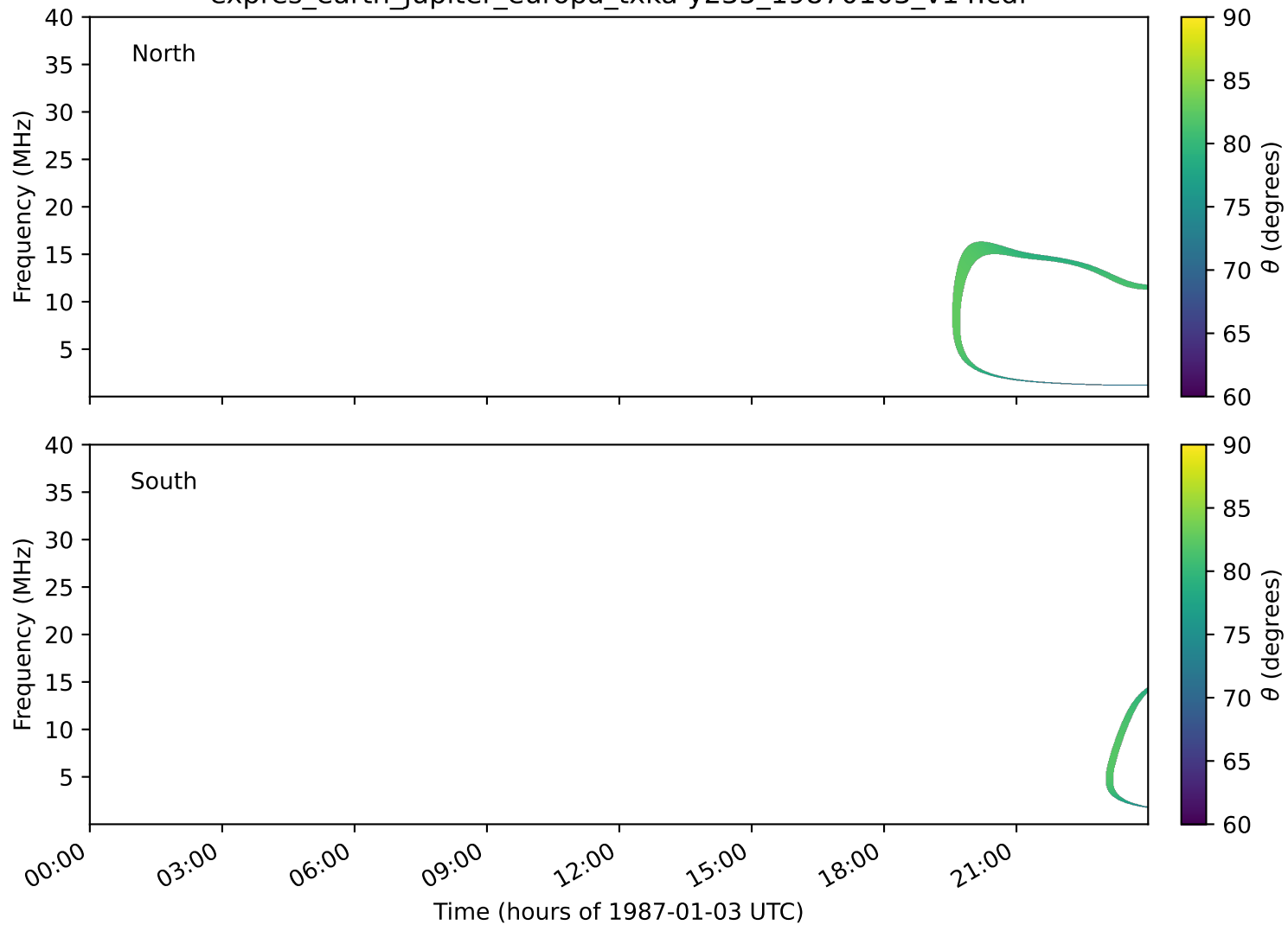
expres_earth_jupiter_europa_txka-y235_19870103_v14.cdf
