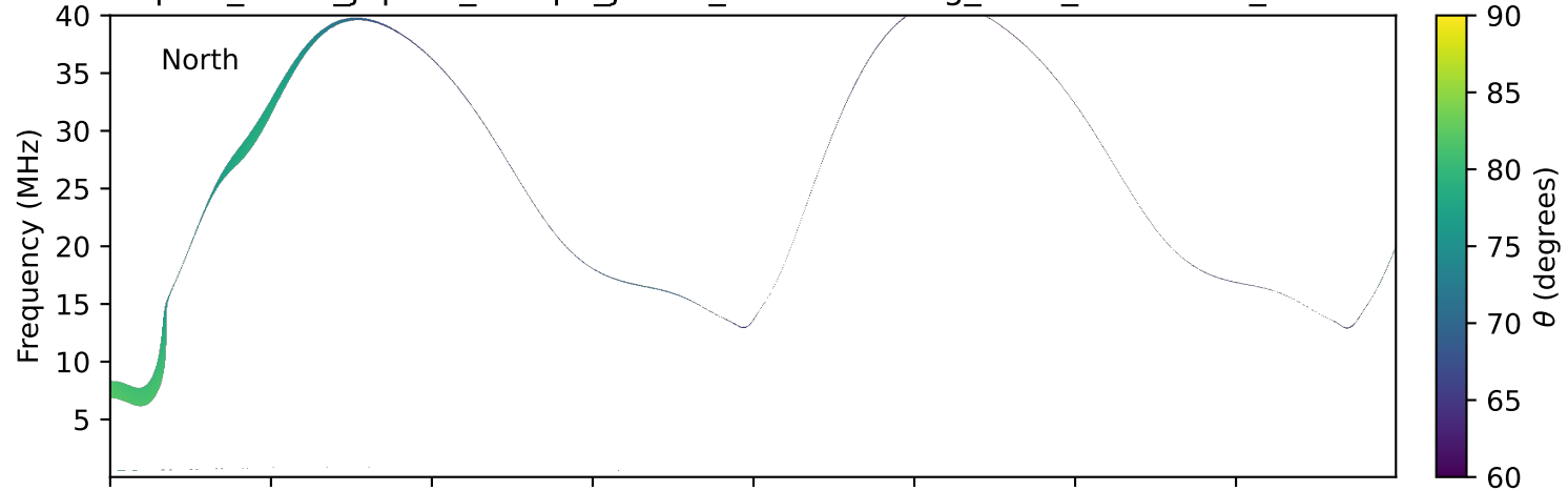
expres_earth_jupiter_europa_jrm09_lossc-wid1deg_3kev_19870104_v11.cdf
