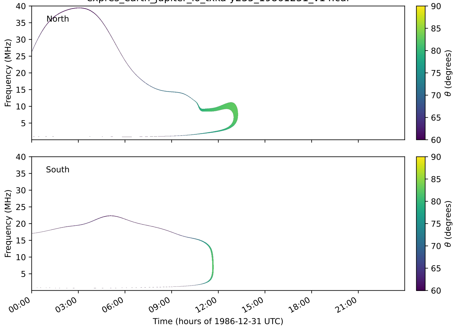
expres_earth_jupiter_io_txka-y235_19861231_v14.cdf
