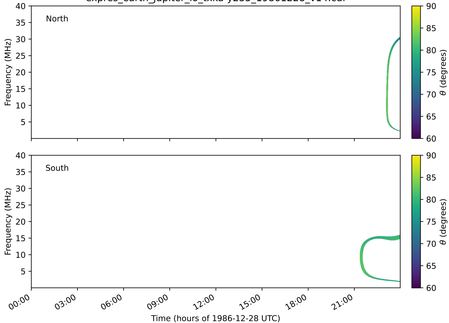
expres_earth_jupiter_io_txka-y235_19861228_v14.cdf
