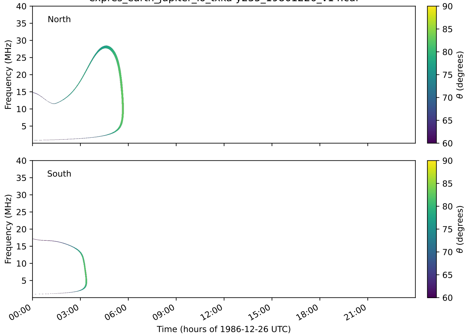
expres_earth_jupiter_io_txka-y235_19861226_v14.cdf
