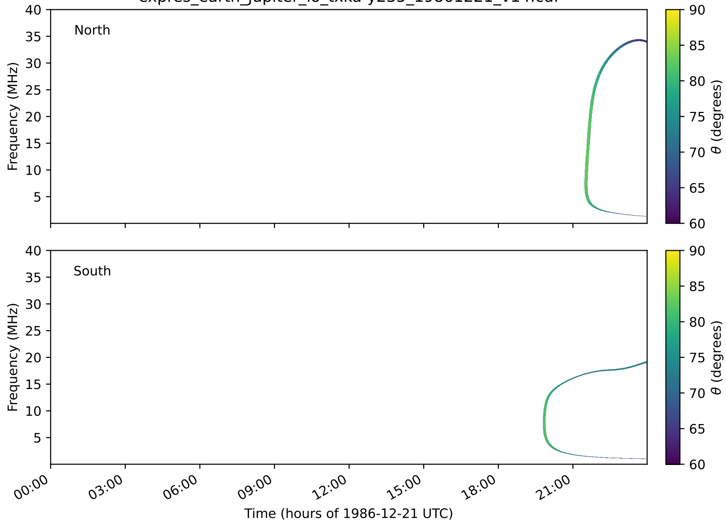
expres_earth_jupiter_io_txka-y235_19861221_v14.cdf
