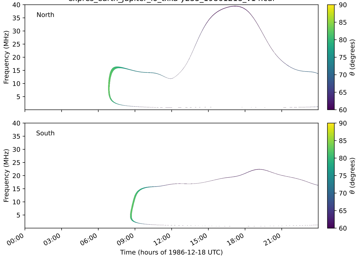
expres_earth_jupiter_io_txka-y235_19861218_v14.cdf
