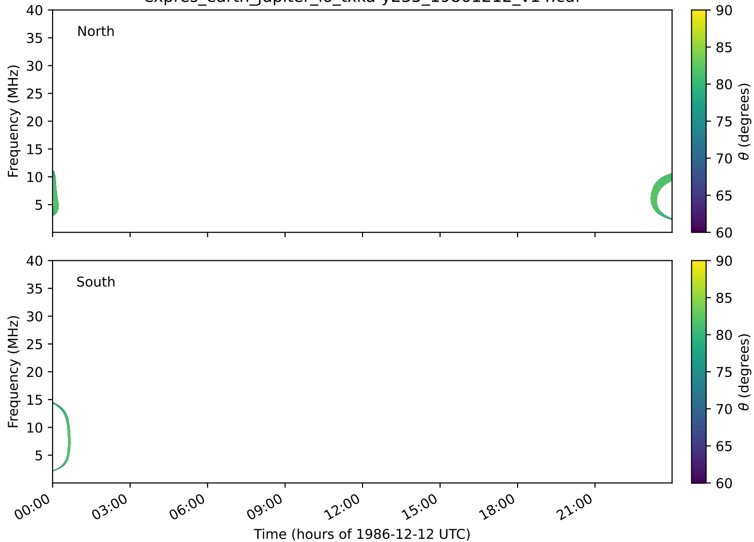
expres_earth_jupiter_io_txka-y235_19861212_v14.cdf
