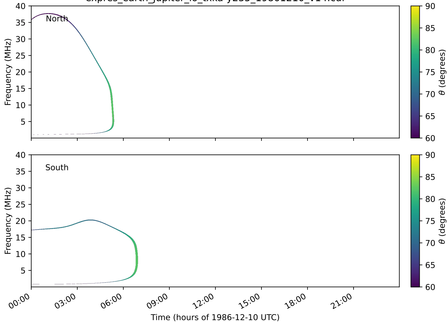
expres_earth_jupiter_io_txka-y235_19861210_v14.cdf
