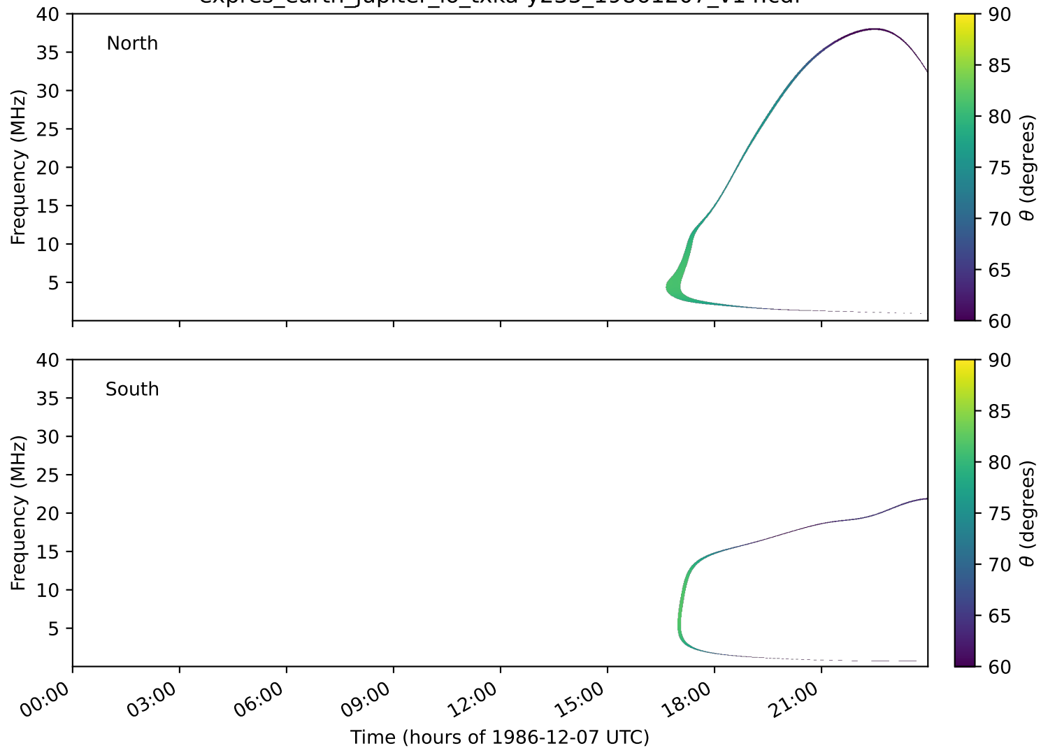
expres_earth_jupiter_io_txka-y235_19861207_v14.cdf
