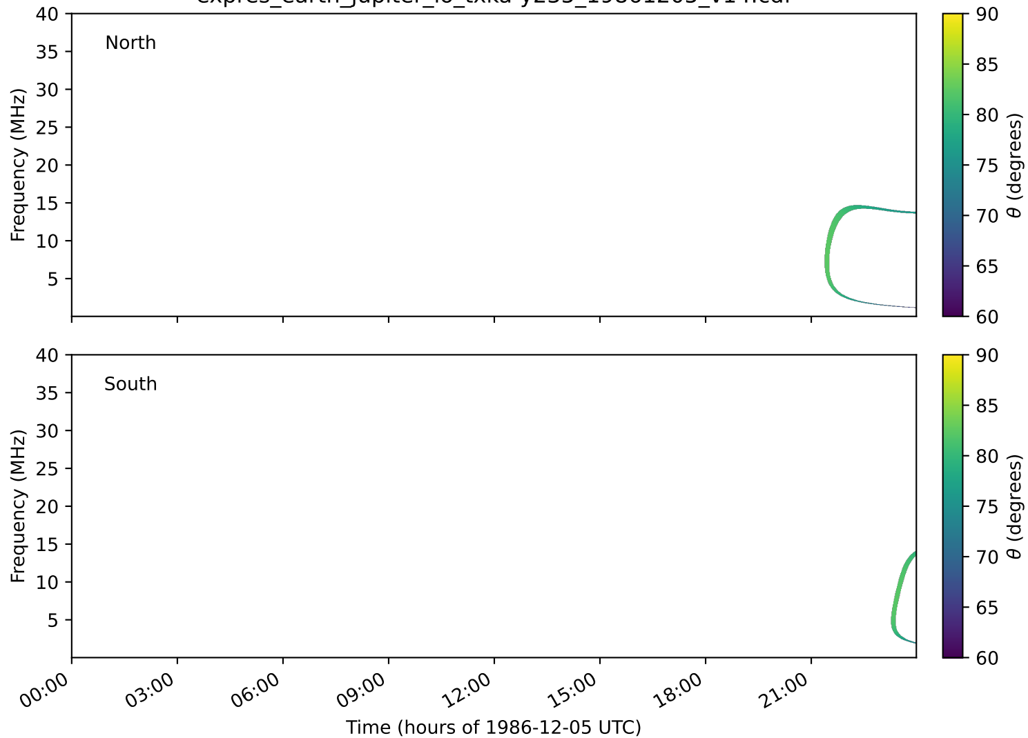
expres_earth_jupiter_io_txka-y235_19861205_v14.cdf
