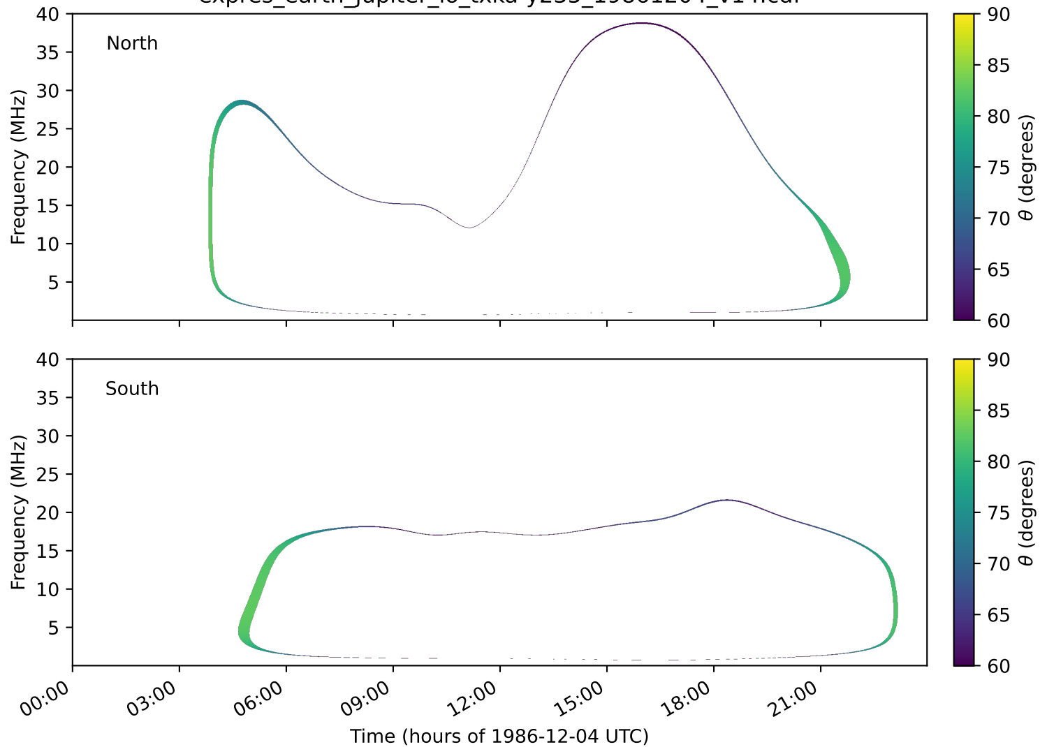
expres_earth_jupiter_io_txka-y235_19861204_v14.cdf
