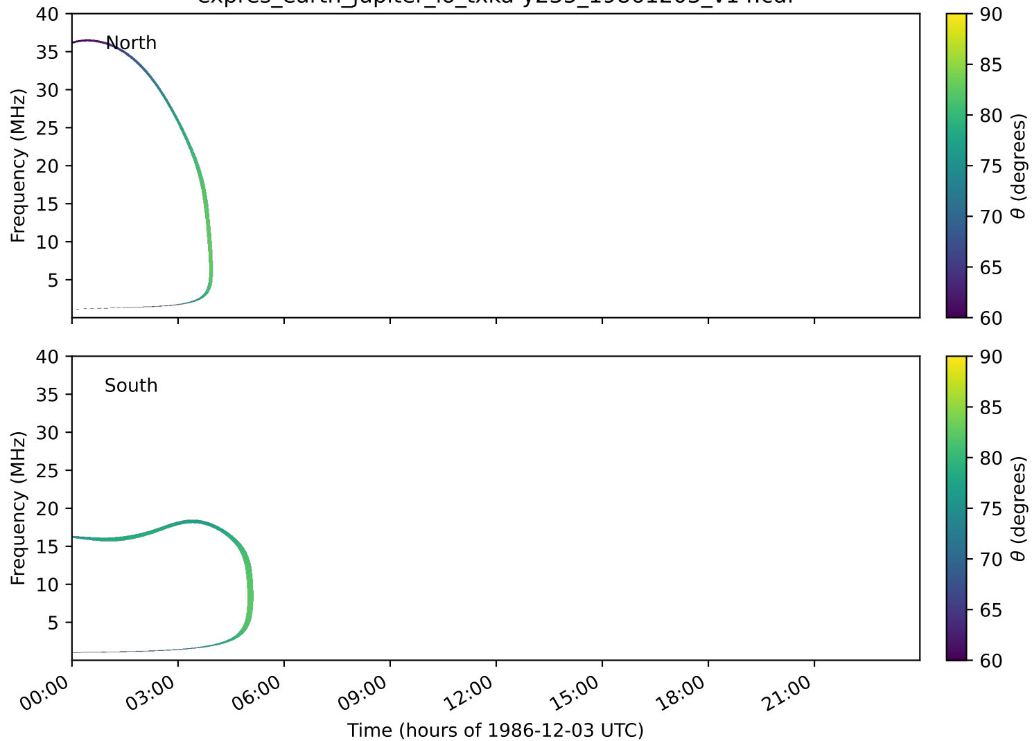
expres_earth_jupiter_io_txka-y235_19861203_v14.cdf
