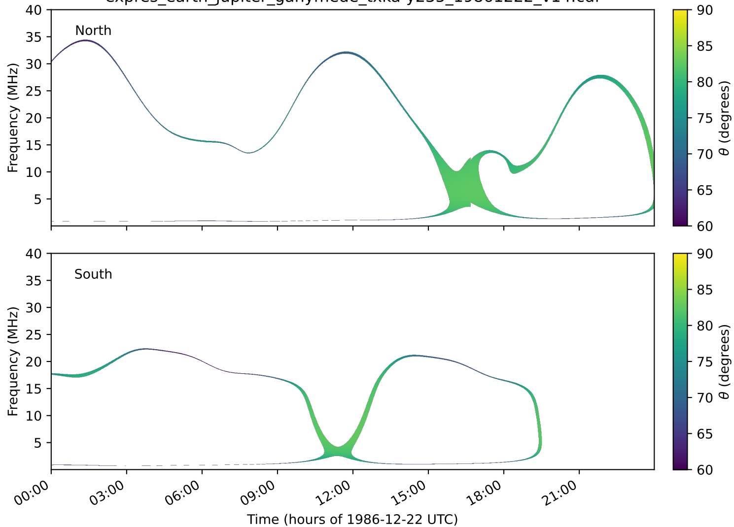
expres_earth_jupiter_ganymede_txka-y235_19861222_v14.cdf
