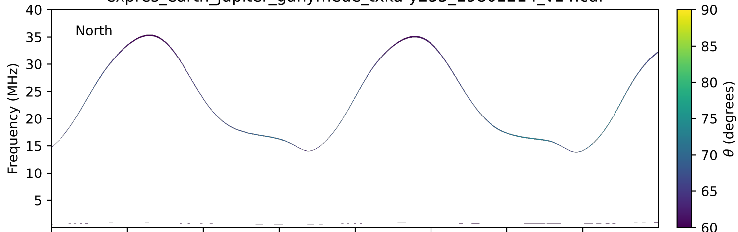
expres_earth_jupiter_ganymede_txka-y235_19861214_v14.cdf
