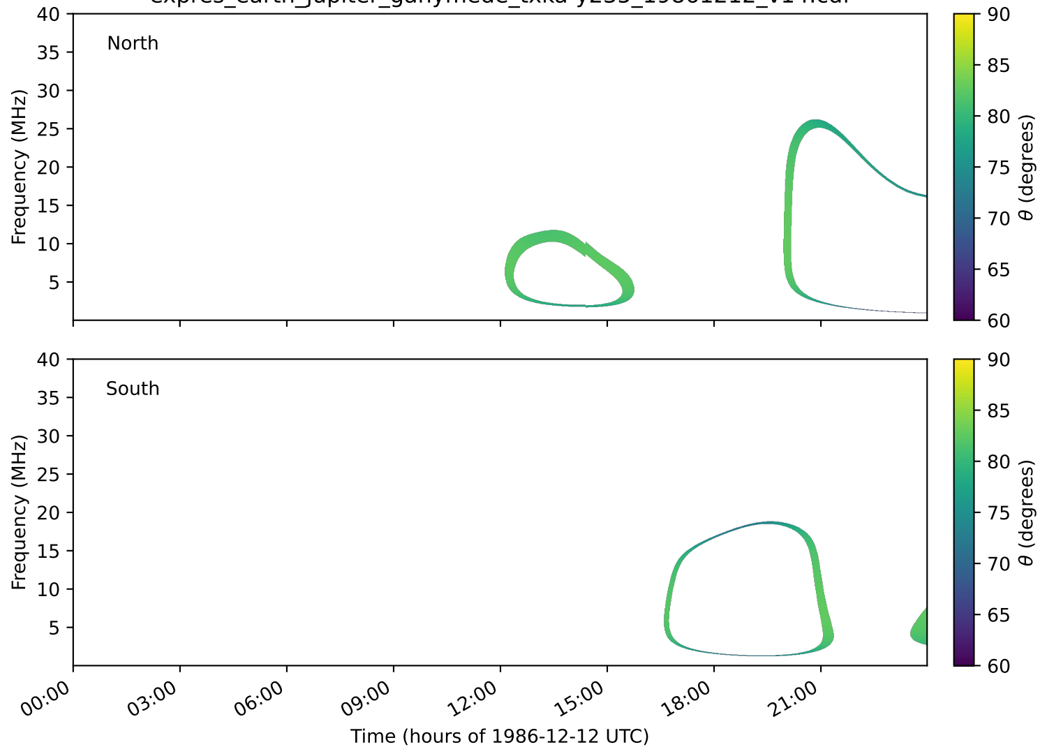
expres_earth_jupiter_ganymede_txka-y235_19861212_v14.cdf
