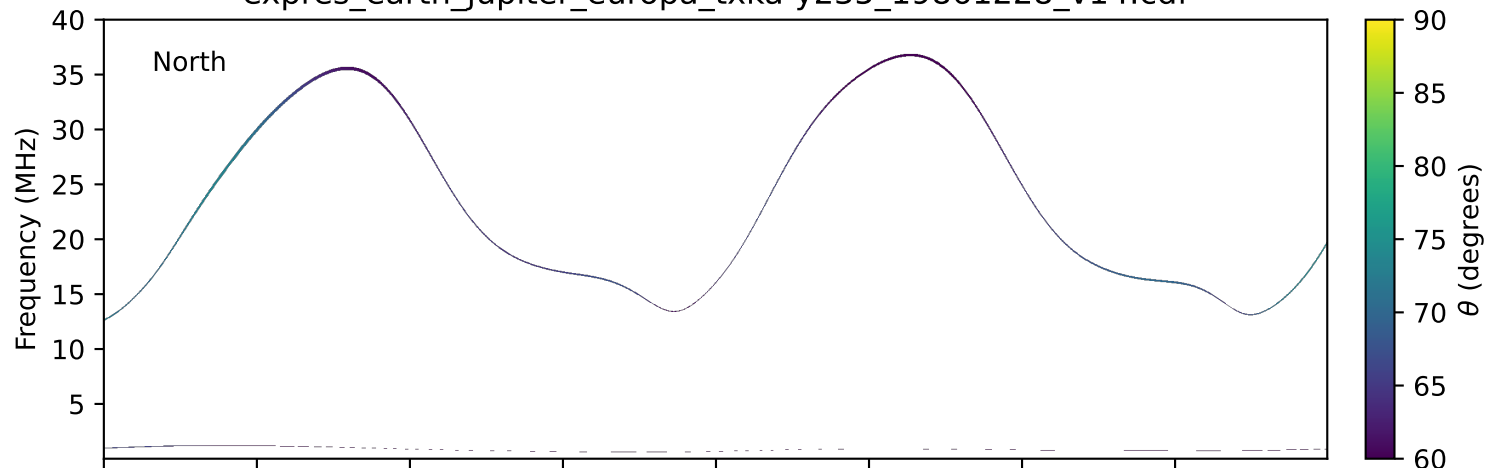
expres_earth_jupiter_europa_txka-y235_19861228_v14.cdf
