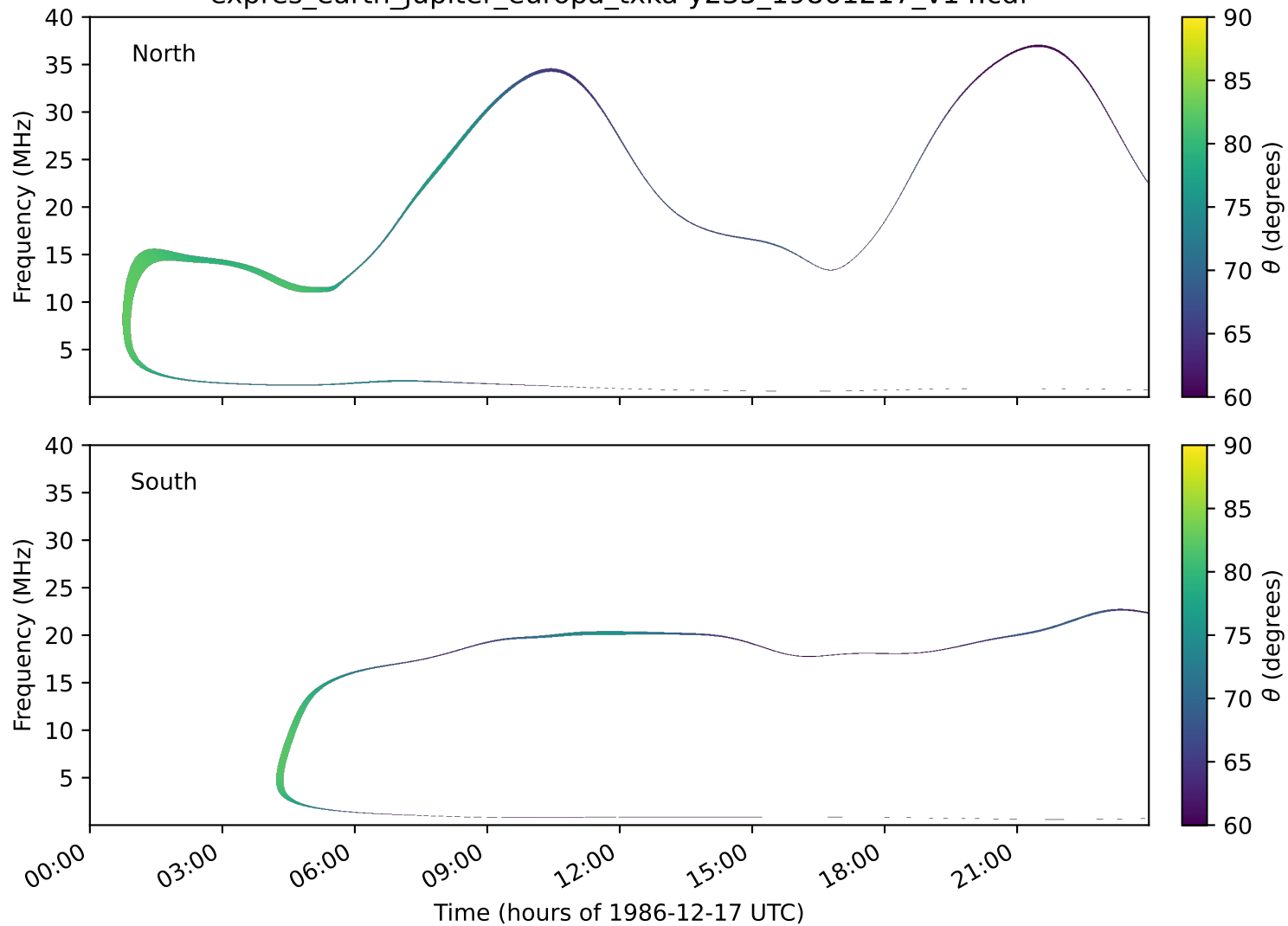
expres_earth_jupiter_europa_txka-y235_19861217_v14.cdf
