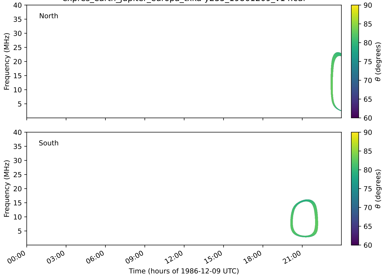
expres_earth_jupiter_europa_txka-y235_19861209_v14.cdf
