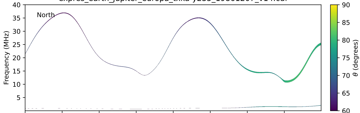
expres_earth_jupiter_europa_txka-y235_19861207_v14.cdf
