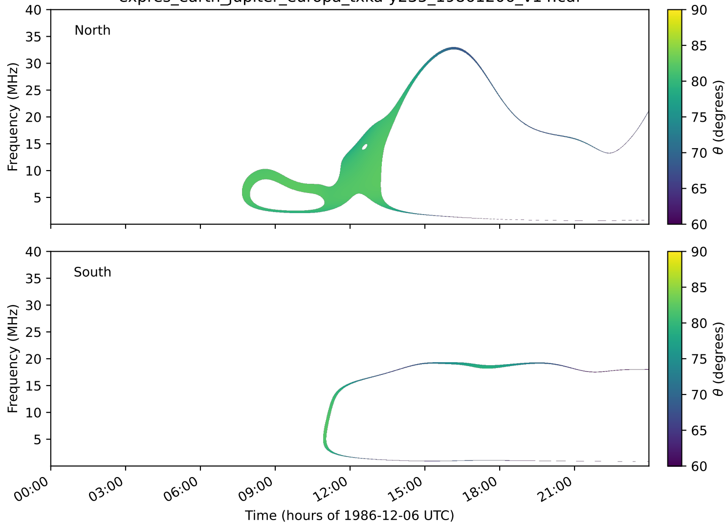
expres_earth_jupiter_europa_txka-y235_19861206_v14.cdf
