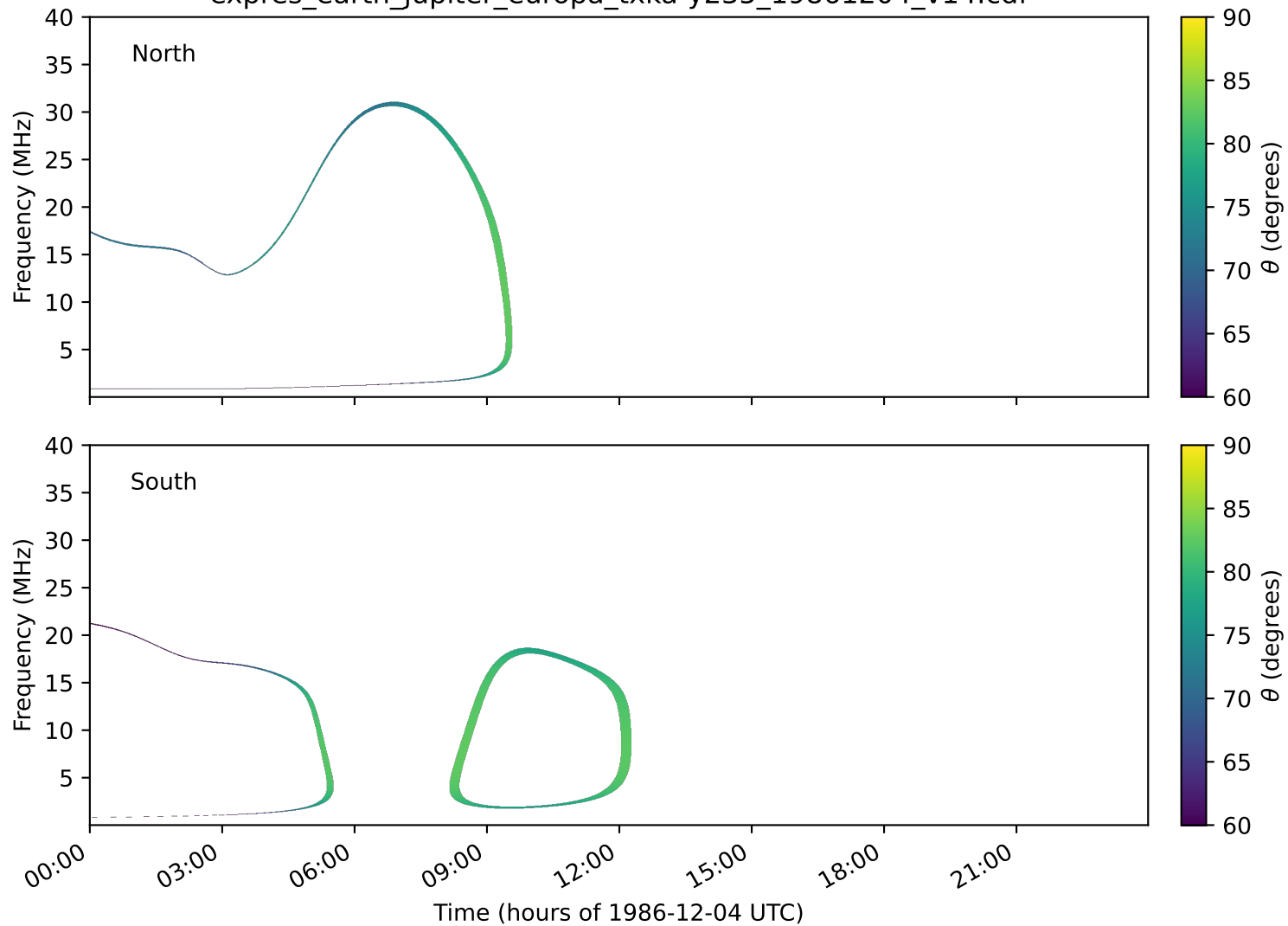
expres_earth_jupiter_europa_txka-y235_19861204_v14.cdf
