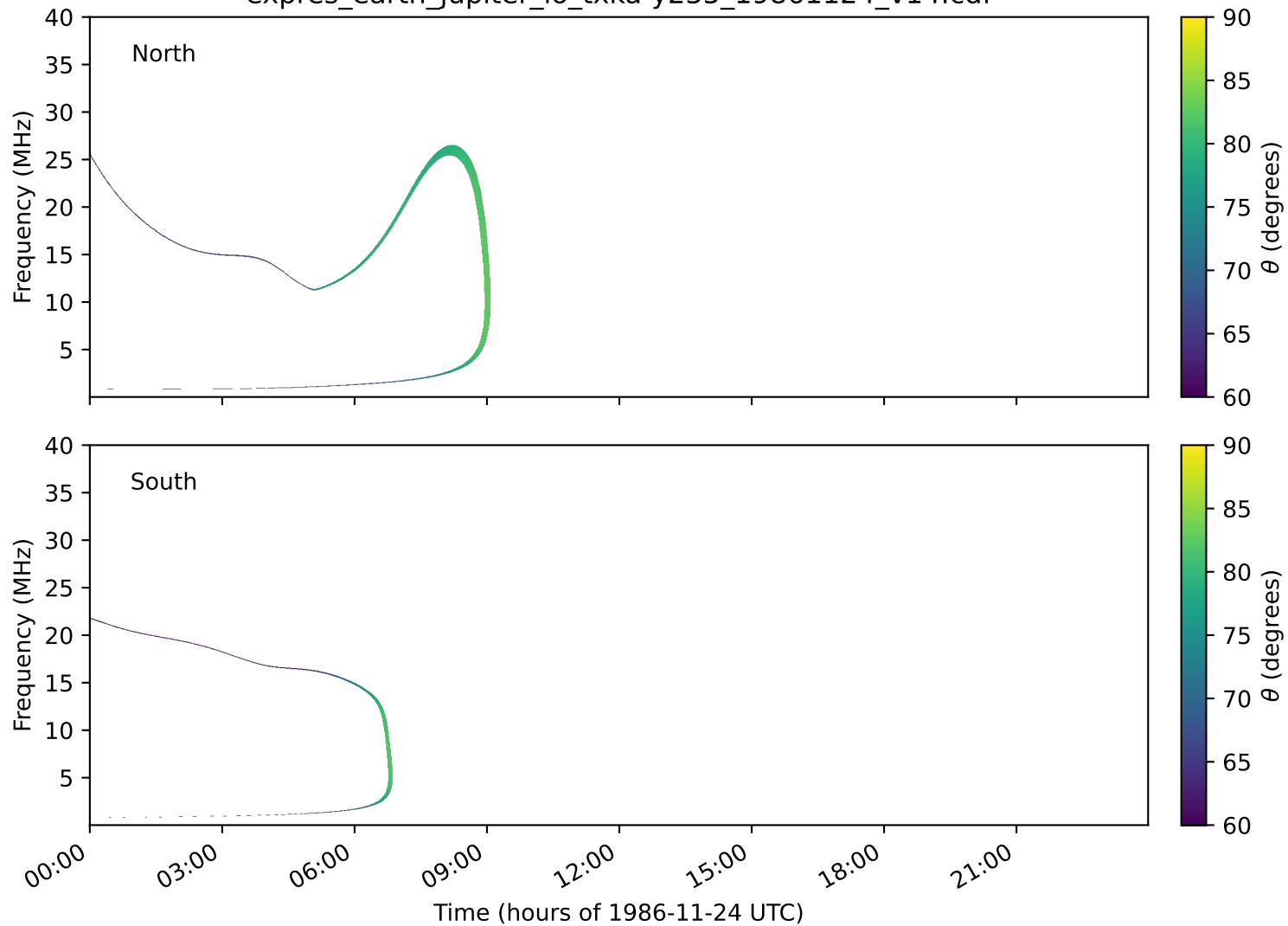
expres_earth_jupiter_io_txka-y235_19861124_v14.cdf
