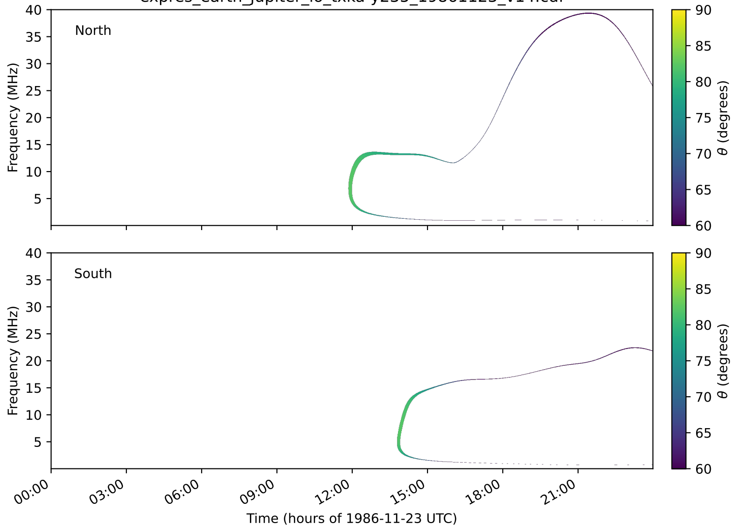
expres_earth_jupiter_io_txka-y235_19861123_v14.cdf
