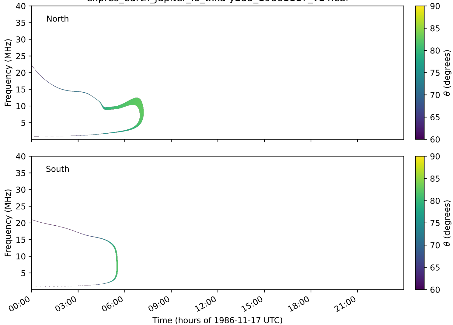
expres_earth_jupiter_io_txka-y235_19861117_v14.cdf
