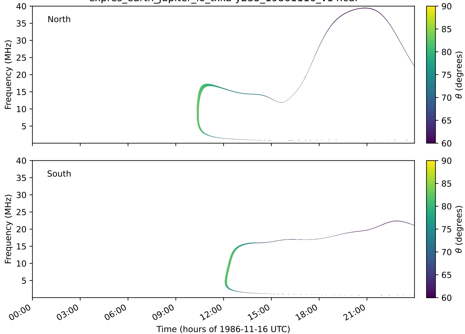
expres_earth_jupiter_io_txka-y235_19861116_v14.cdf
