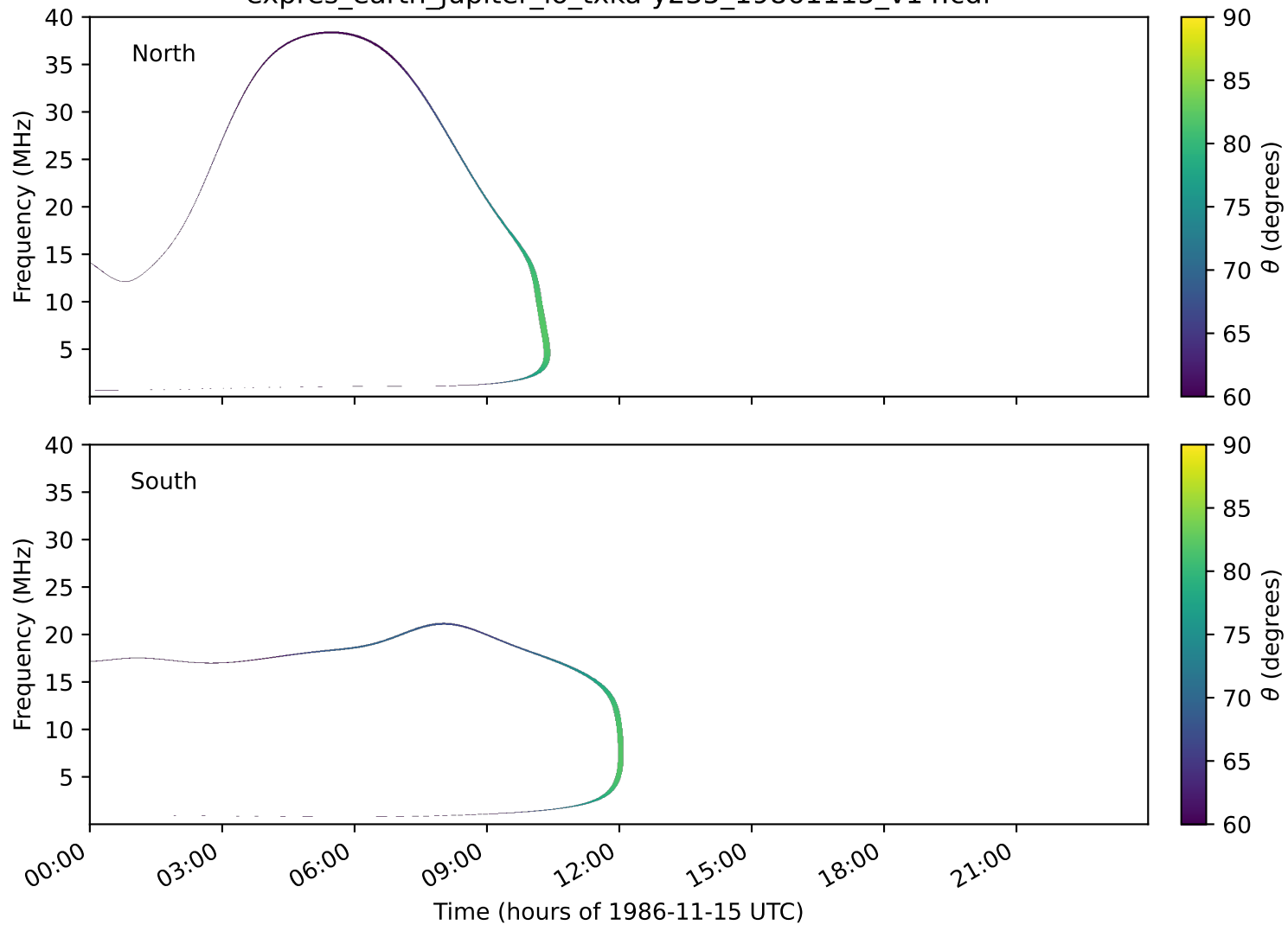
expres_earth_jupiter_io_txka-y235_19861115_v14.cdf
