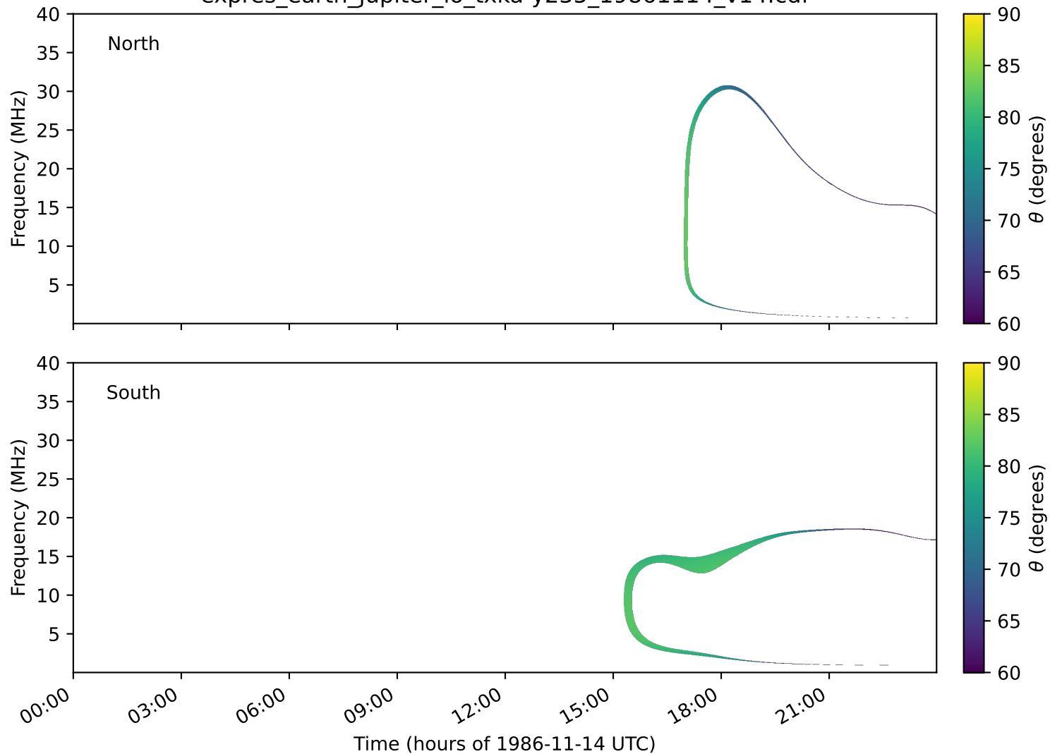
expres_earth_jupiter_io_txka-y235_19861114_v14.cdf
