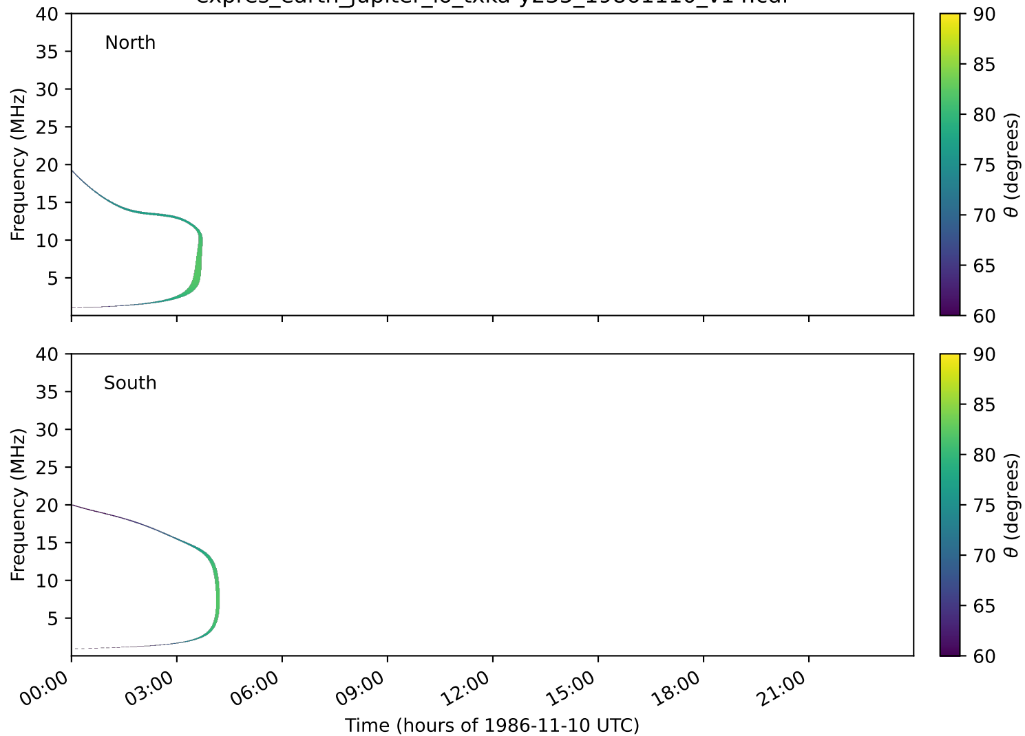
expres_earth_jupiter_io_txka-y235_19861110_v14.cdf
