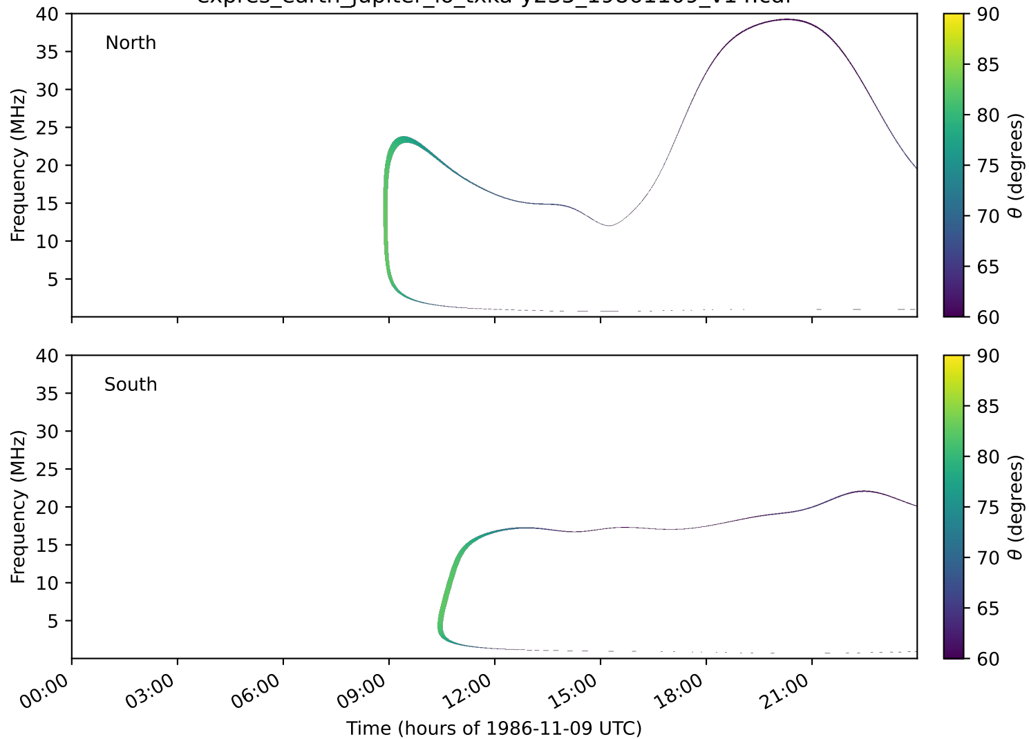
expres_earth_jupiter_io_txka-y235_19861109_v14.cdf
