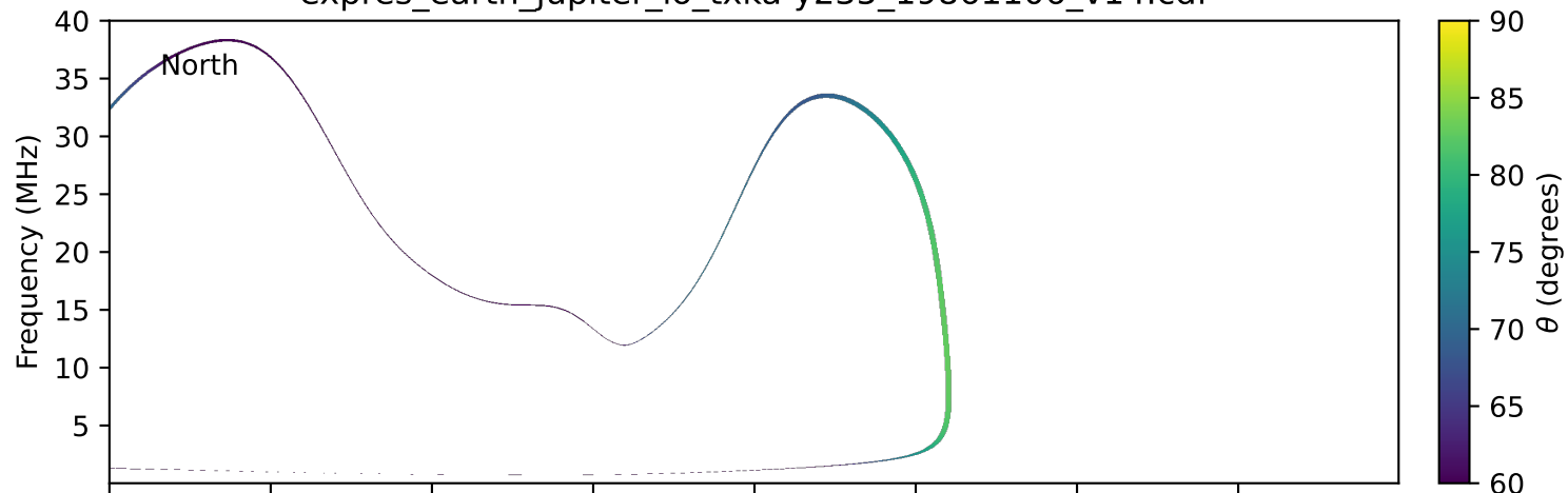
expres_earth_jupiter_io_txka-y235_19861106_v14.cdf
