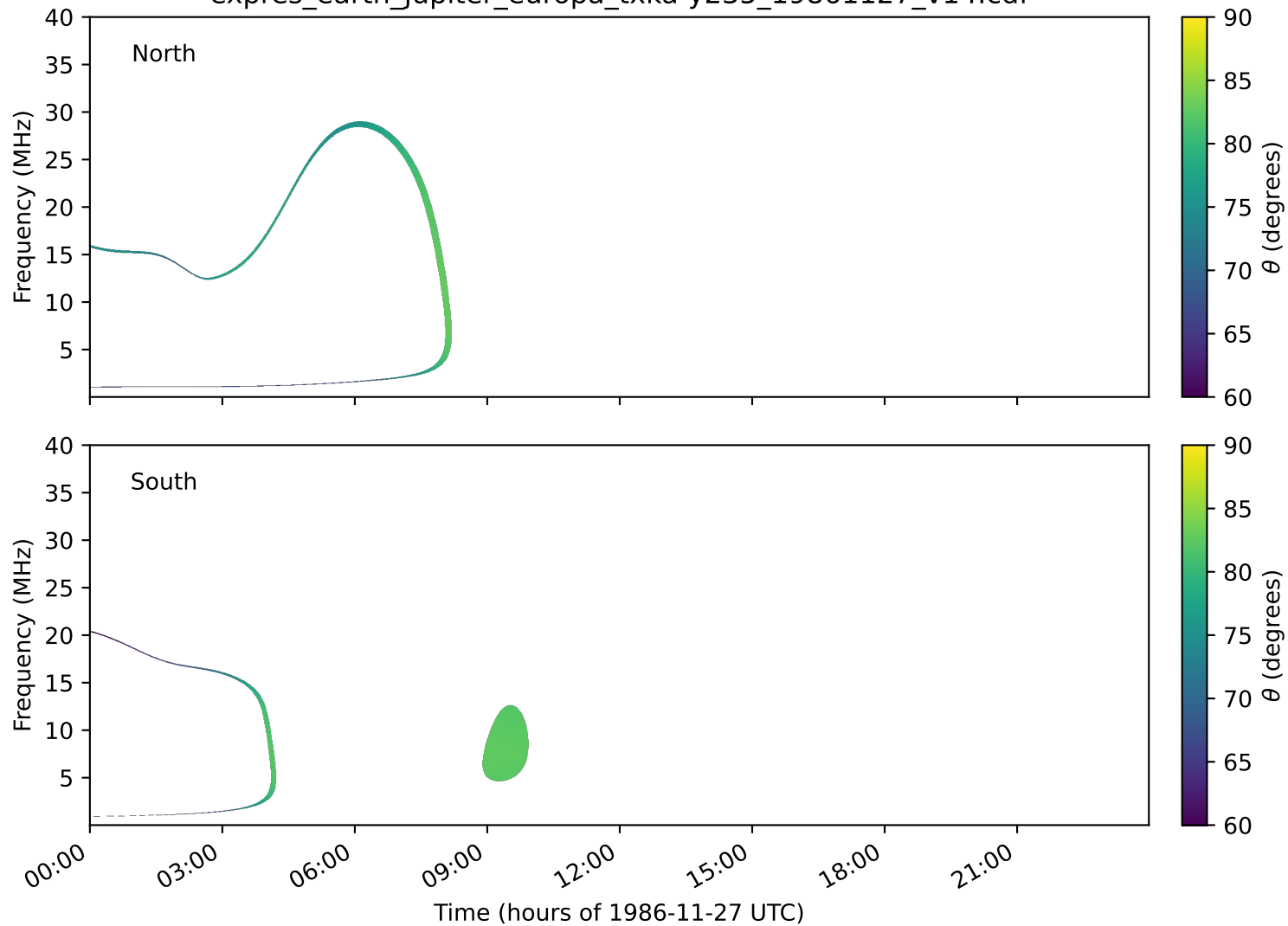
expres_earth_jupiter_europa_txka-y235_19861127_v14.cdf
