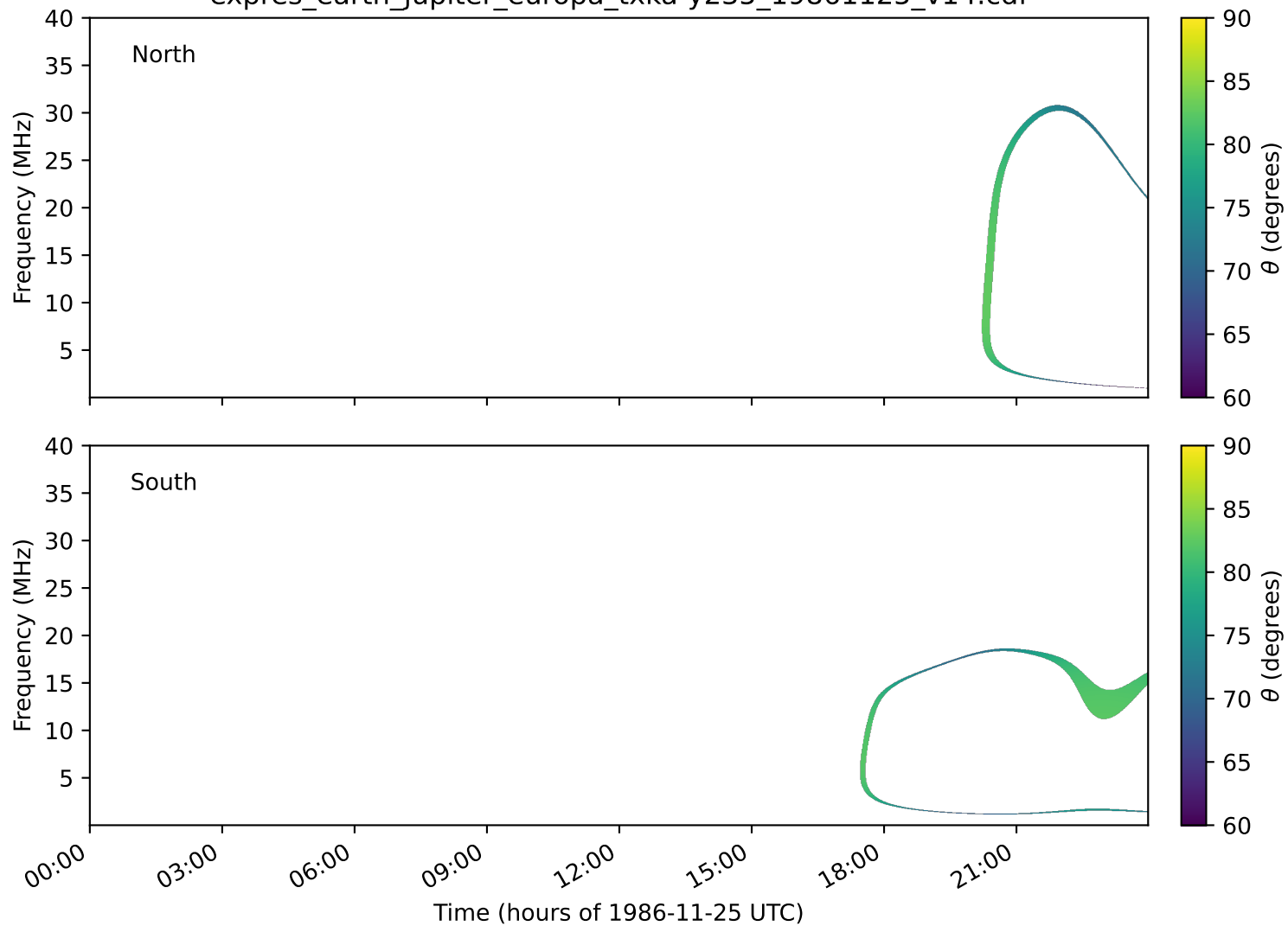
expres_earth_jupiter_europa_txka-y235_19861125_v14.cdf
