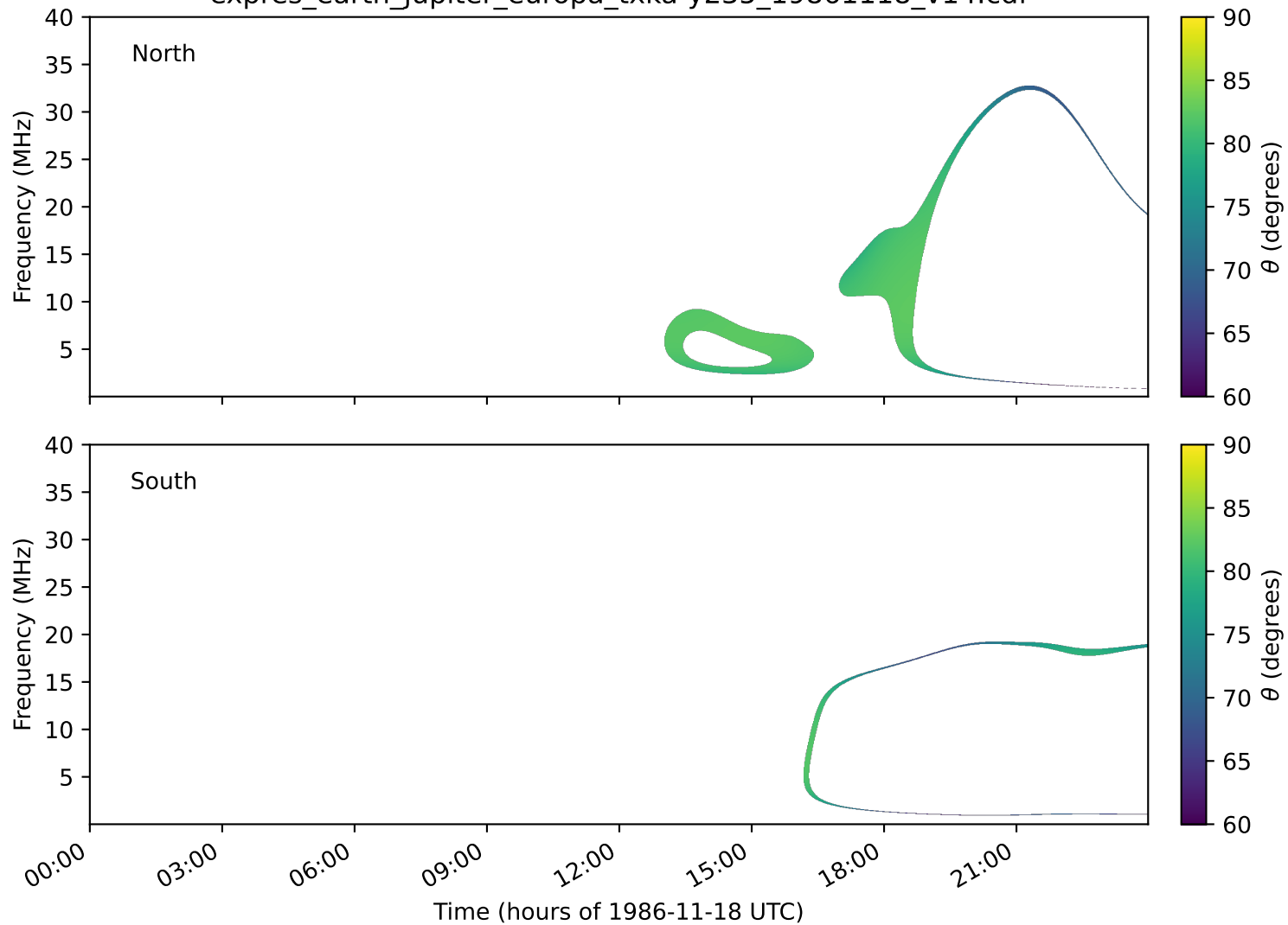
expres_earth_jupiter_europa_txka-y235_19861118_v14.cdf
