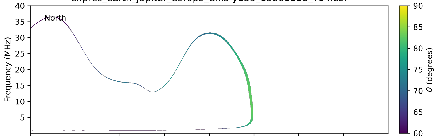
expres_earth_jupiter_europa_txka-y235_19861116_v14.cdf
