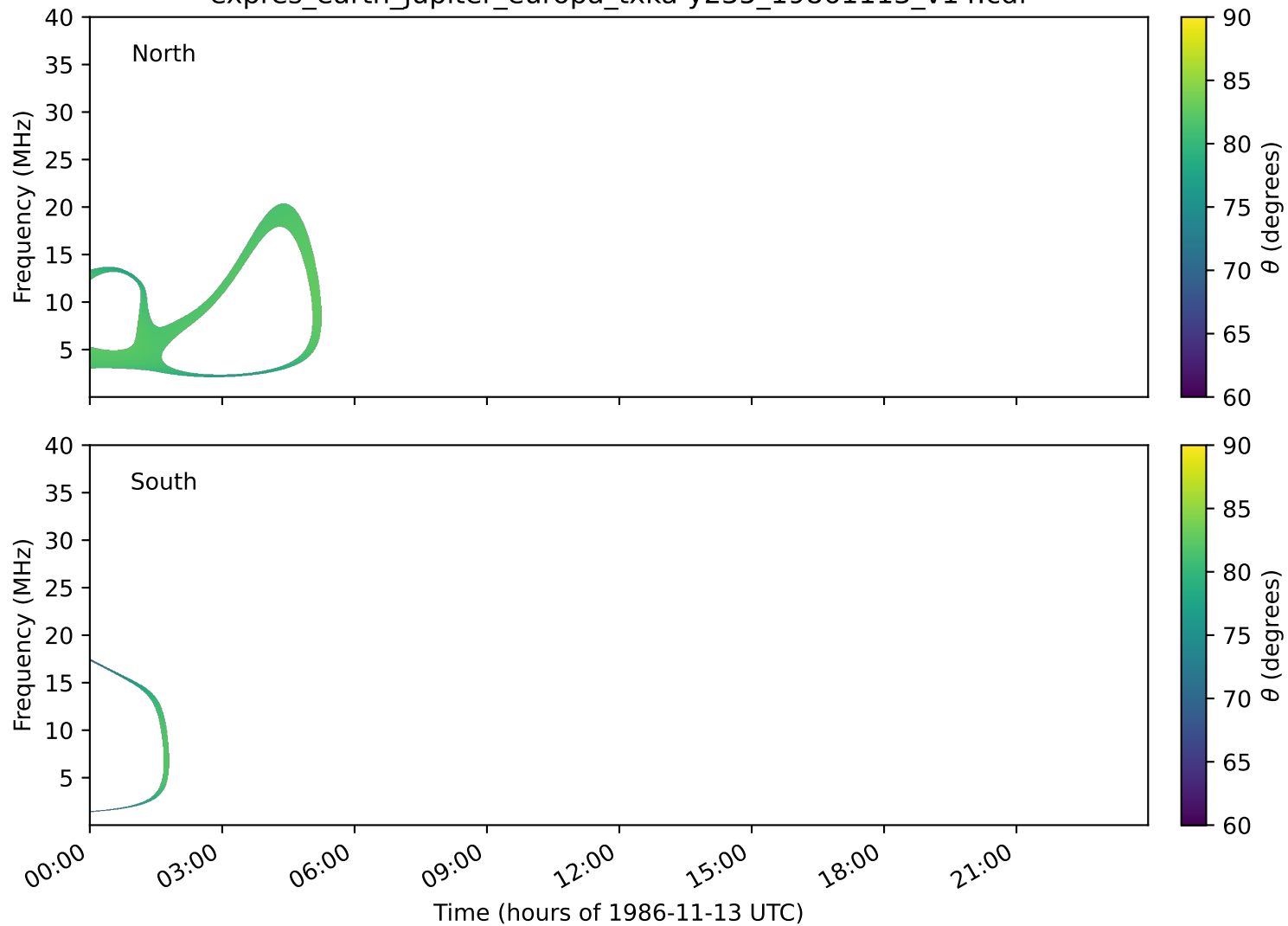
expres_earth_jupiter_europa_txka-y235_19861113_v14.cdf
