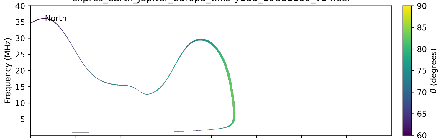
expres_earth_jupiter_europa_txka-y235_19861109_v14.cdf
