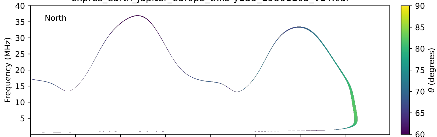
expres_earth_jupiter_europa_txka-y235_19861105_v14.cdf
