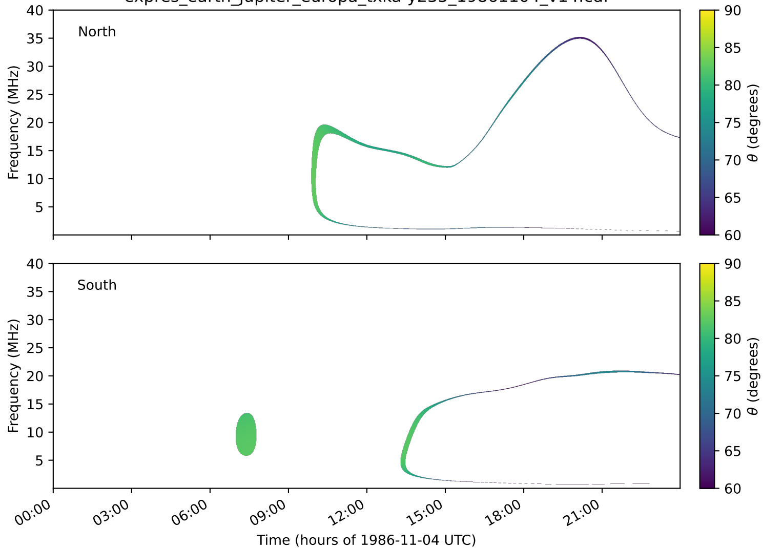
expres_earth_jupiter_europa_txka-y235_19861104_v14.cdf
