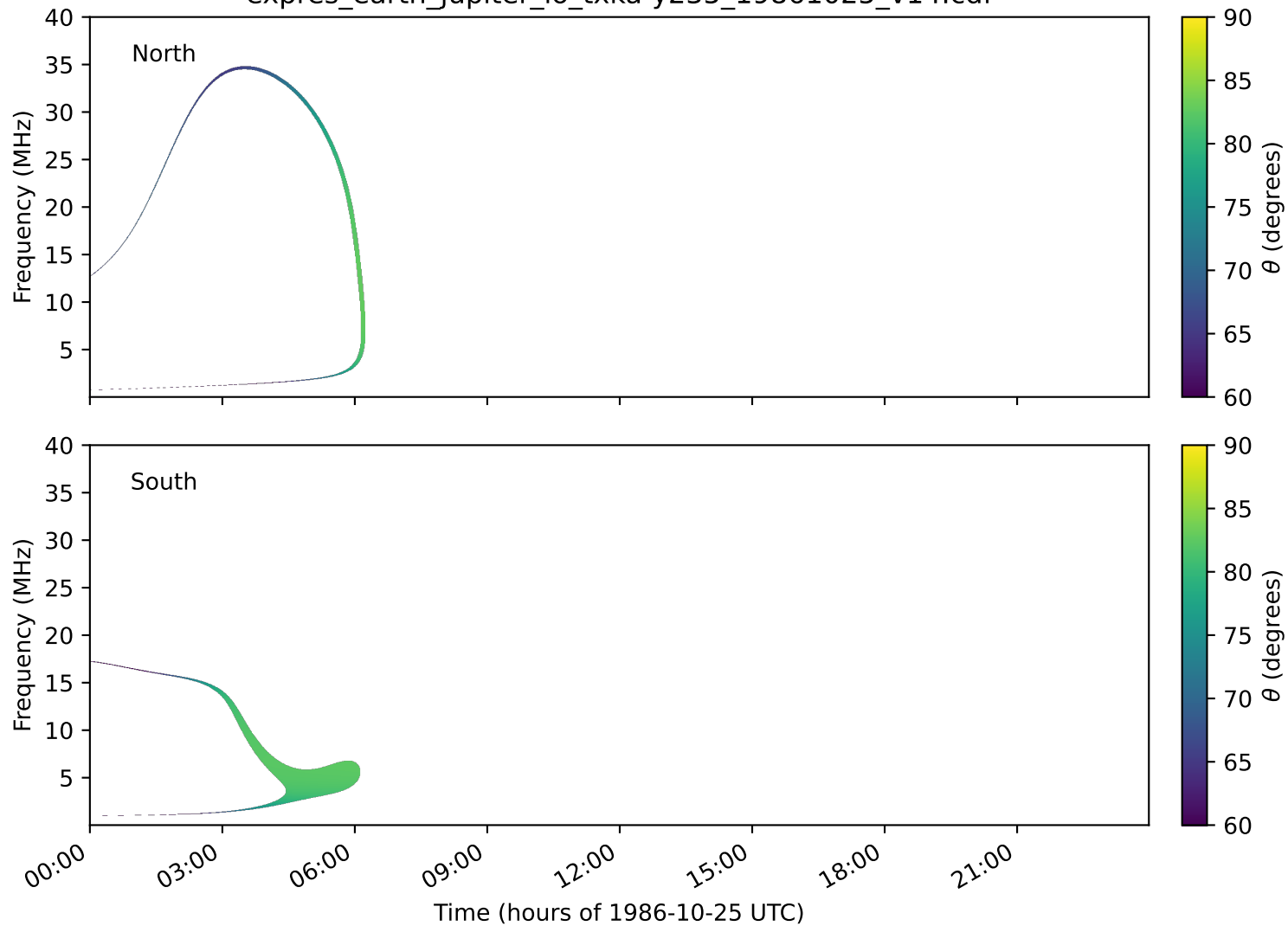
expres_earth_jupiter_io_txka-y235_19861025_v14.cdf
