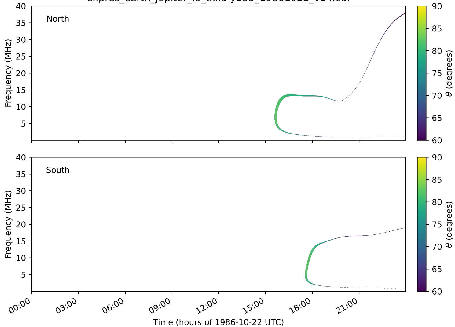
expres_earth_jupiter_io_txka-y235_19861022_v14.cdf
