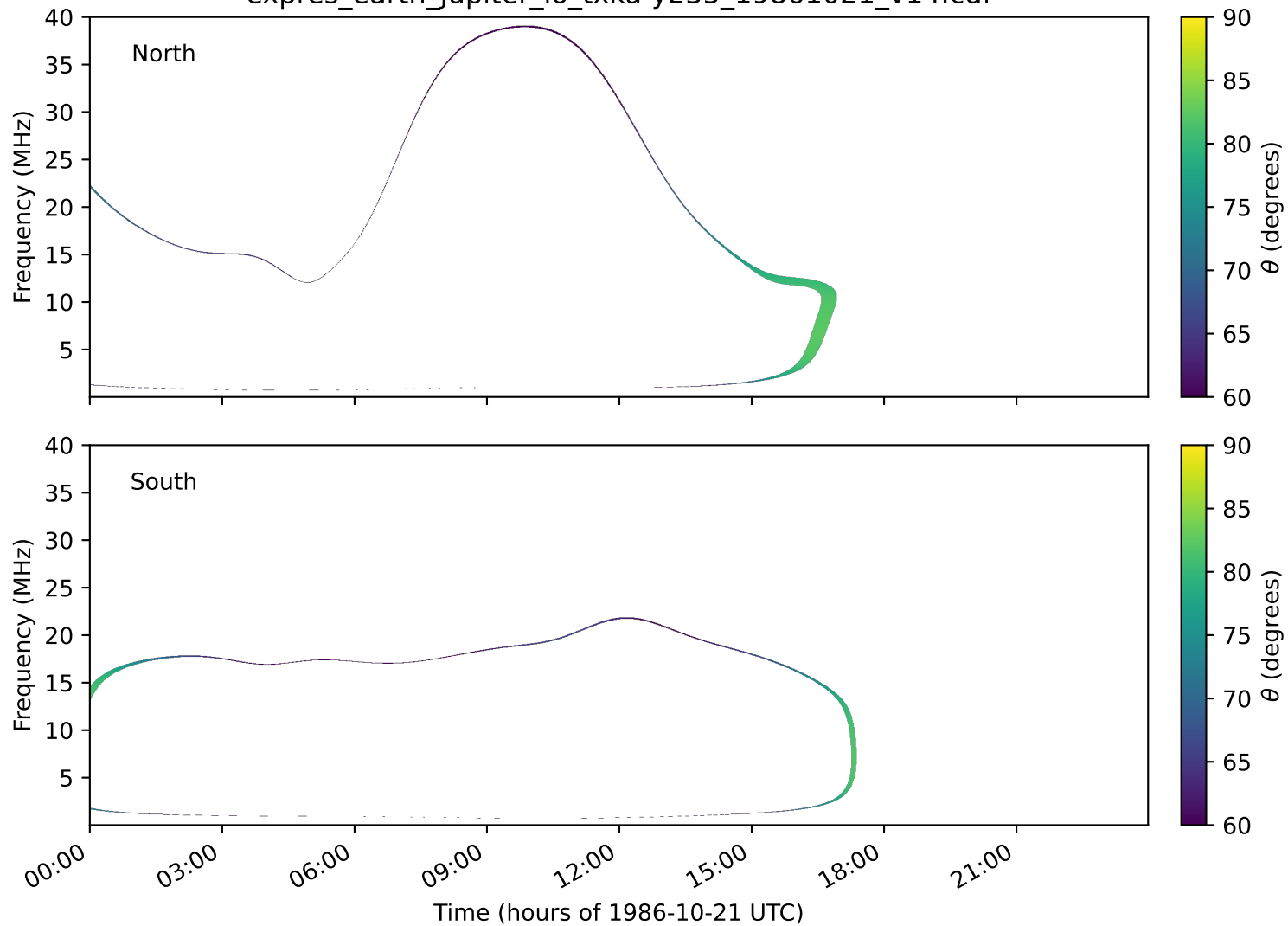
expres_earth_jupiter_io_txka-y235_19861021_v14.cdf
