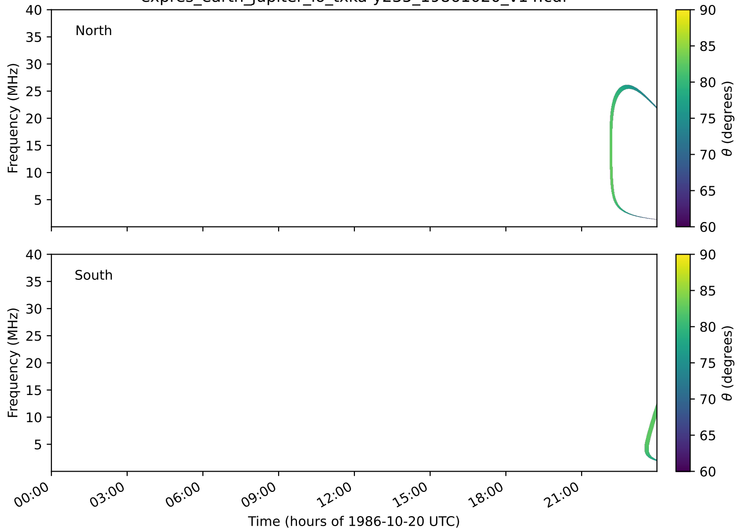
expres_earth_jupiter_io_txka-y235_19861020_v14.cdf
