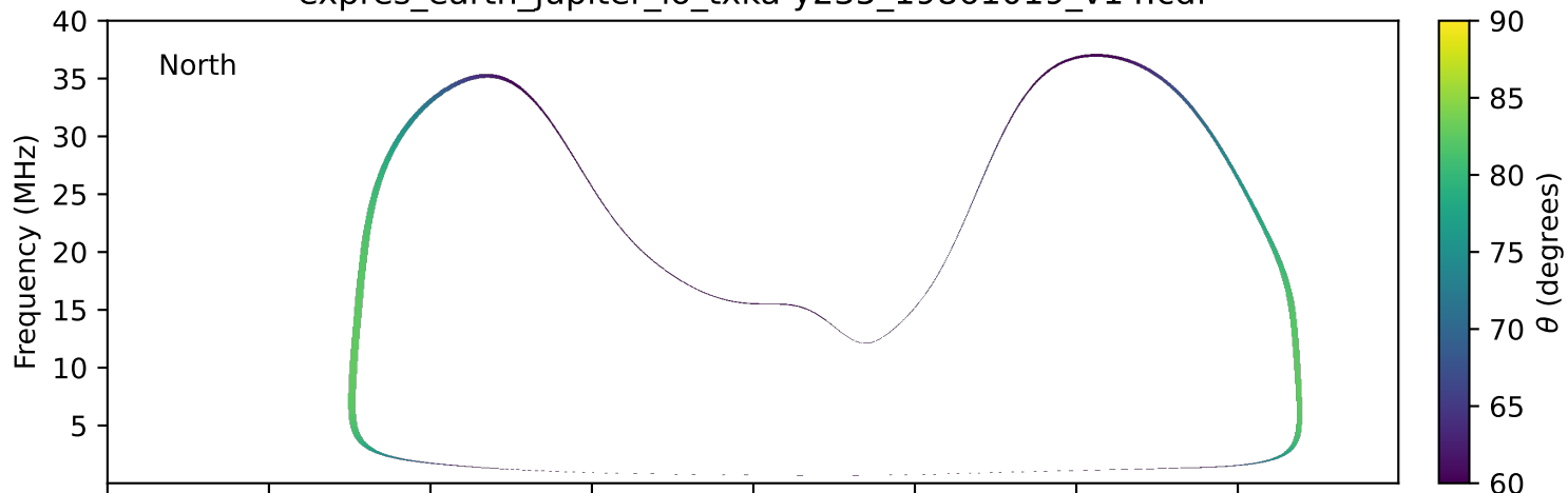
expres_earth_jupiter_io_txka-y235_19861019_v14.cdf
