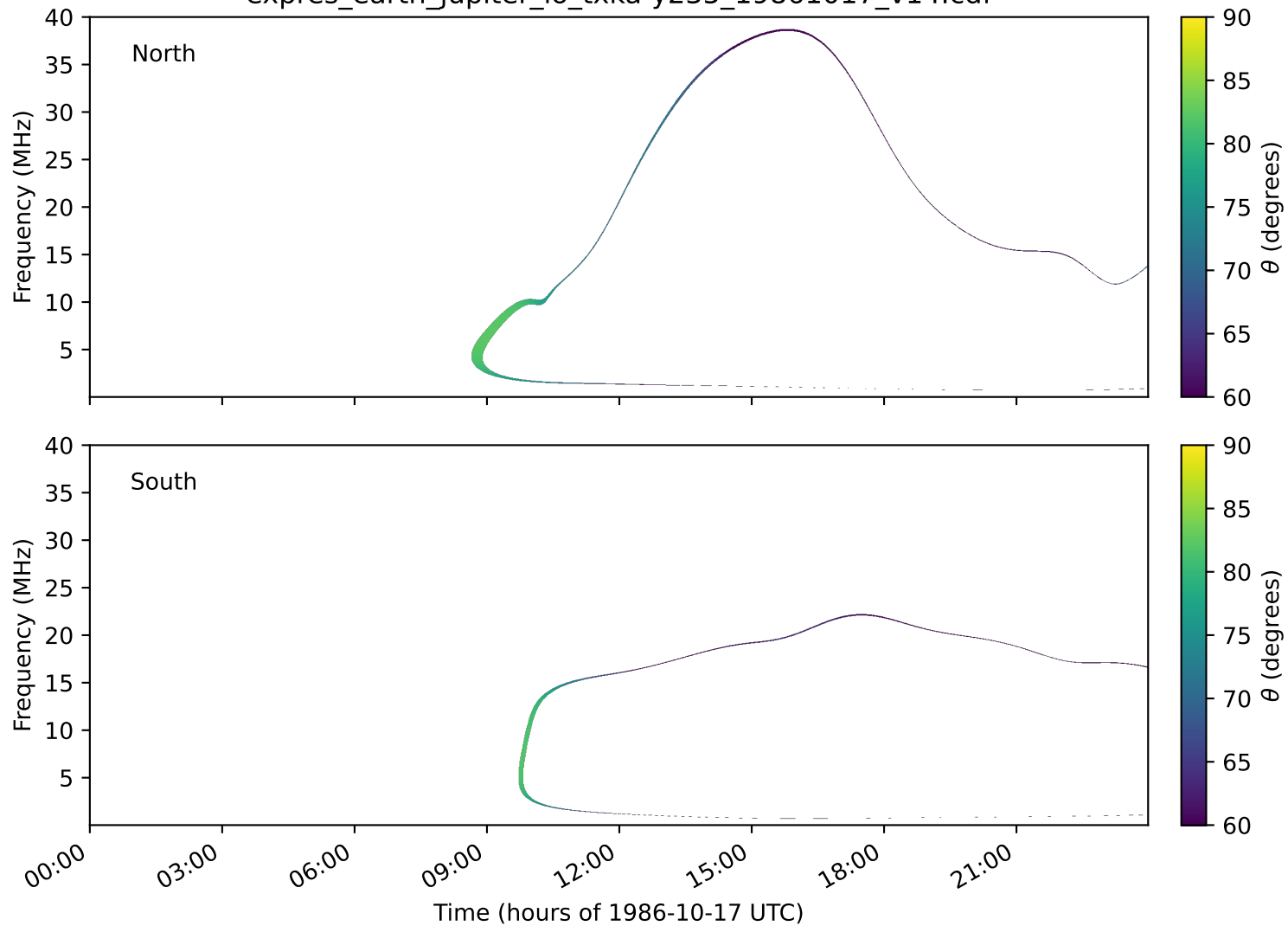
expres_earth_jupiter_io_txka-y235_19861017_v14.cdf
