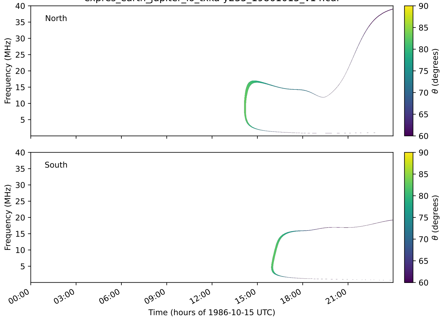
expres_earth_jupiter_io_txka-y235_19861015_v14.cdf
