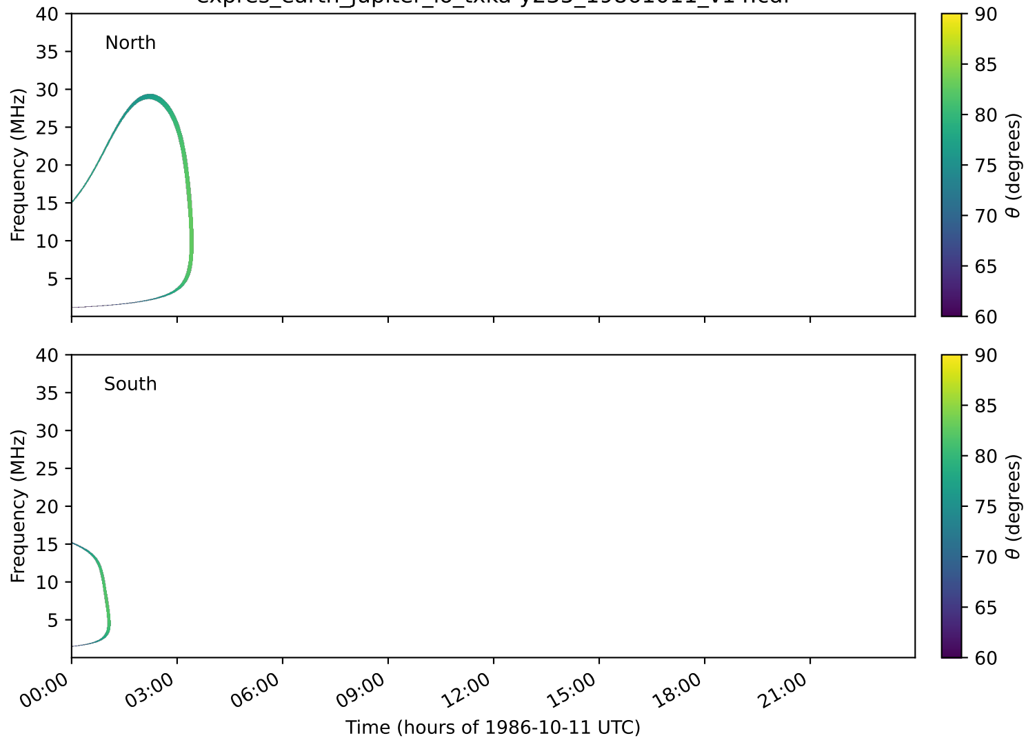
expres_earth_jupiter_io_txka-y235_19861011_v14.cdf
