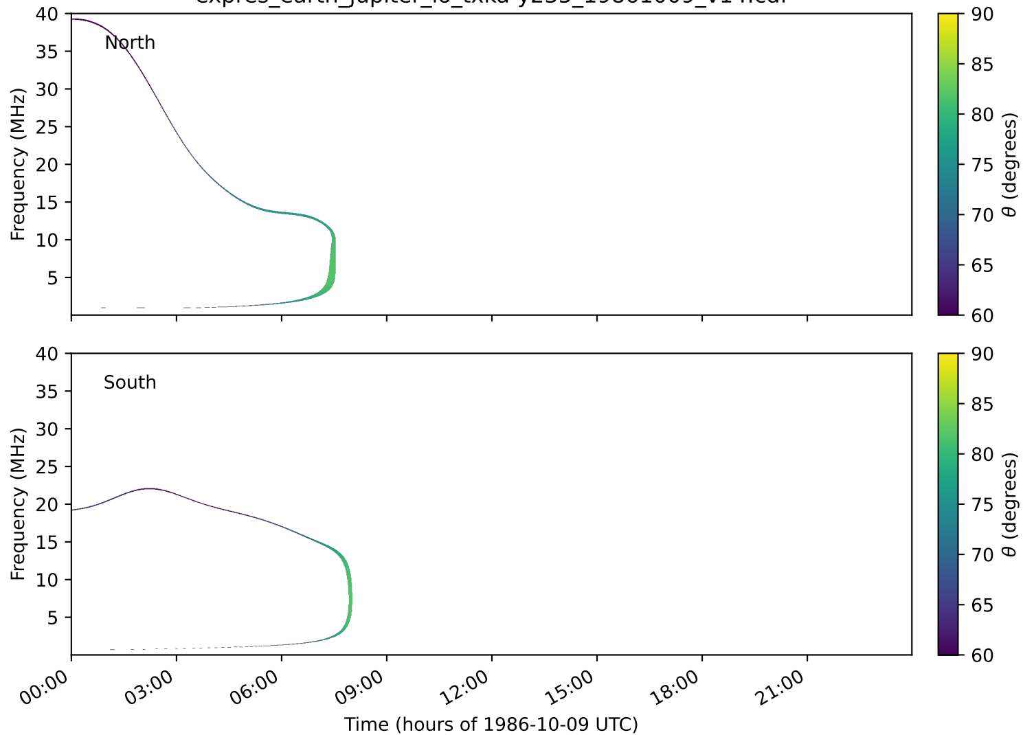
expres_earth_jupiter_io_txka-y235_19861009_v14.cdf
