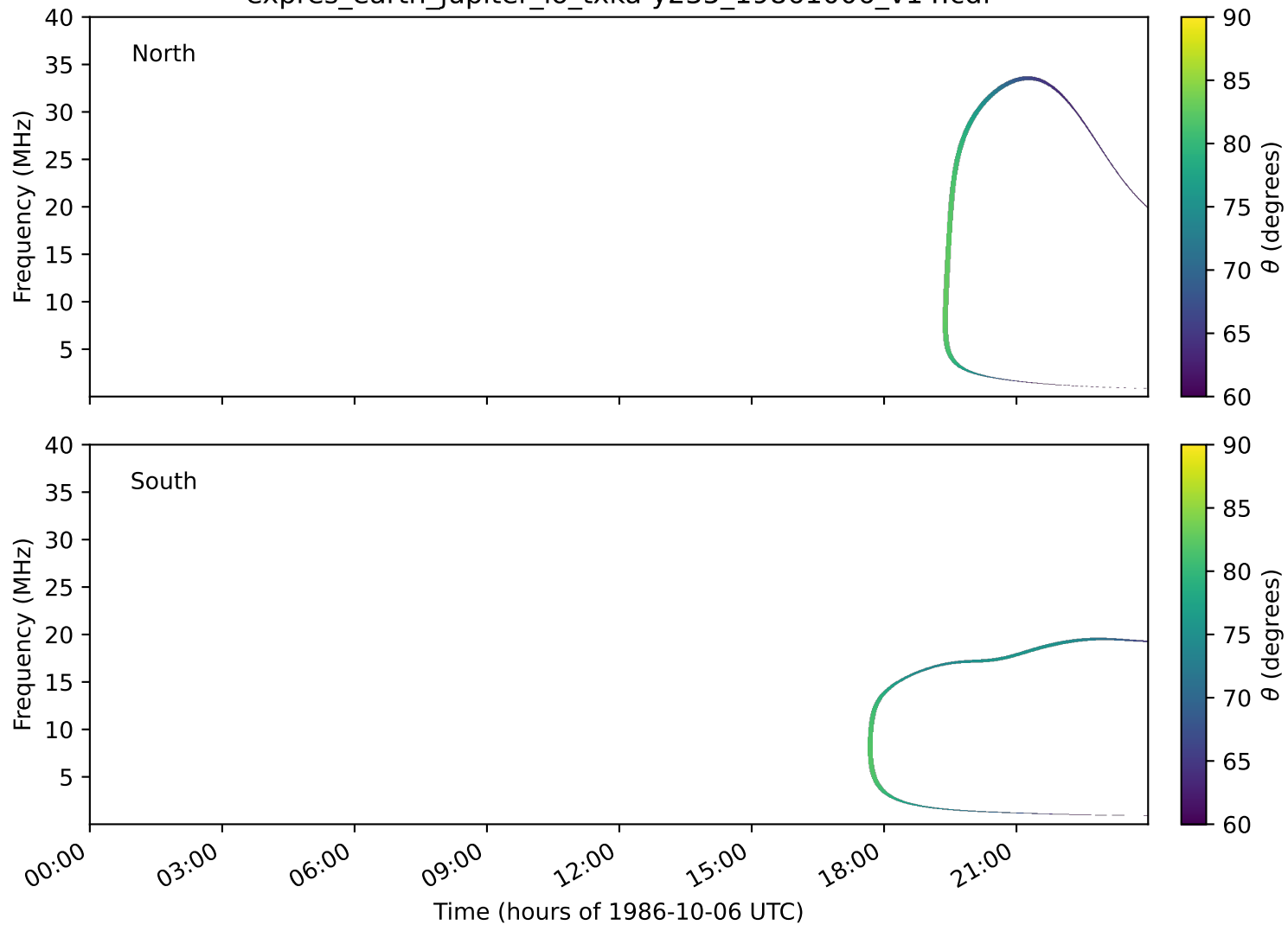
expres_earth_jupiter_io_txka-y235_19861006_v14.cdf
